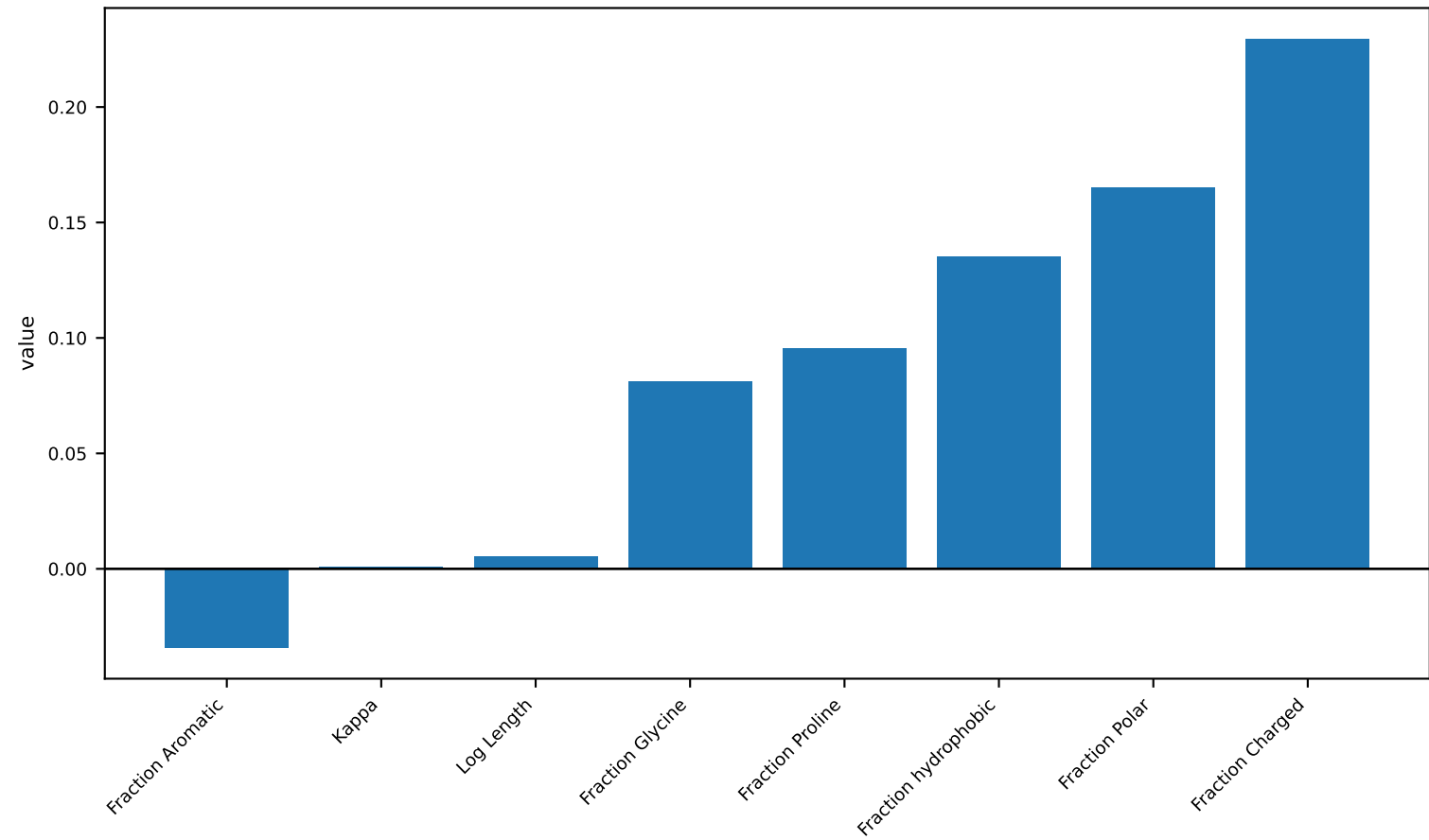
Linear regression feature coefficients
