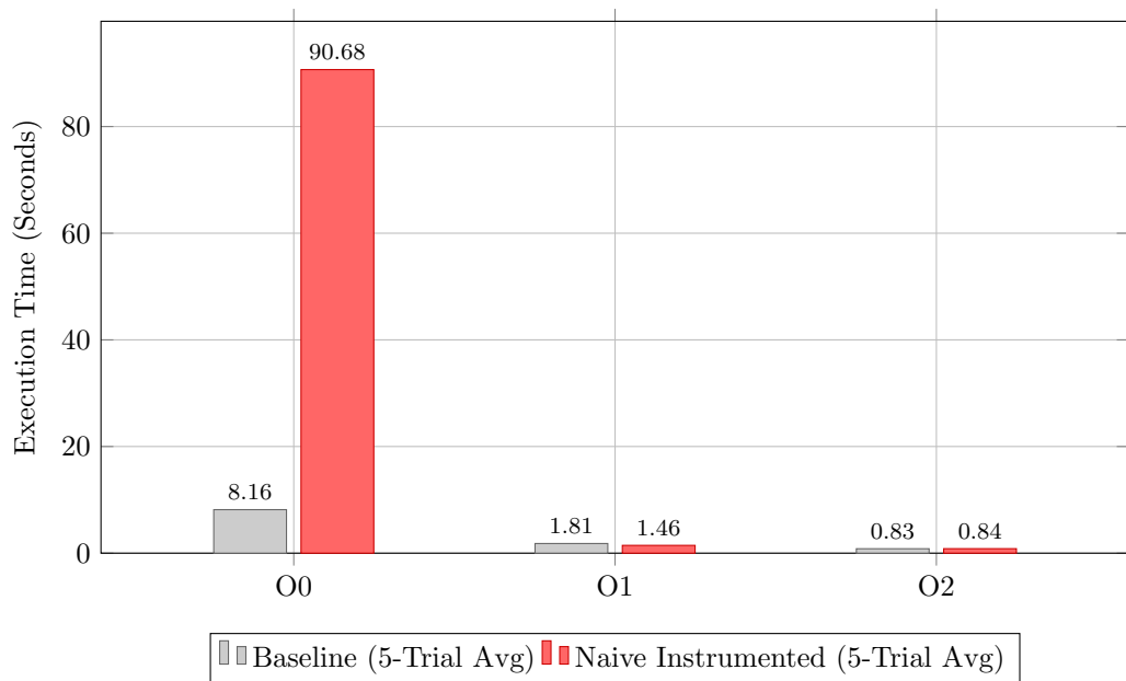
Execution Time: Naive Instrumentation (matmult-int)
