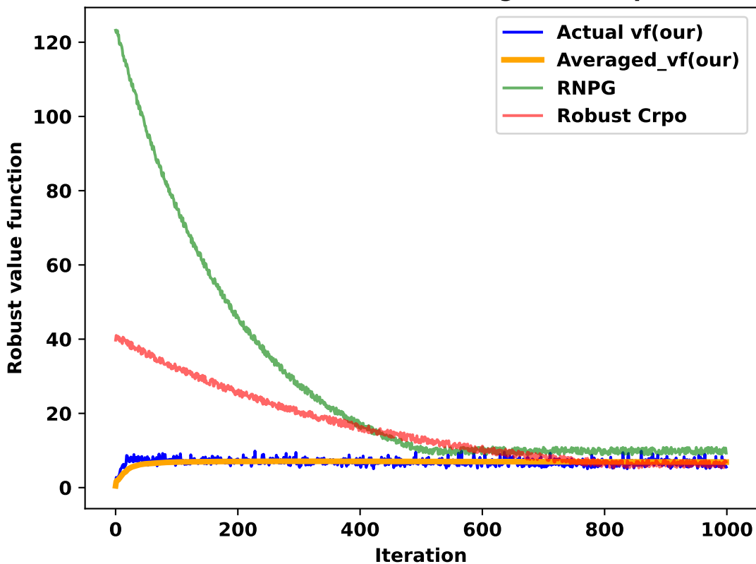
Value function for RVI in augmented space
