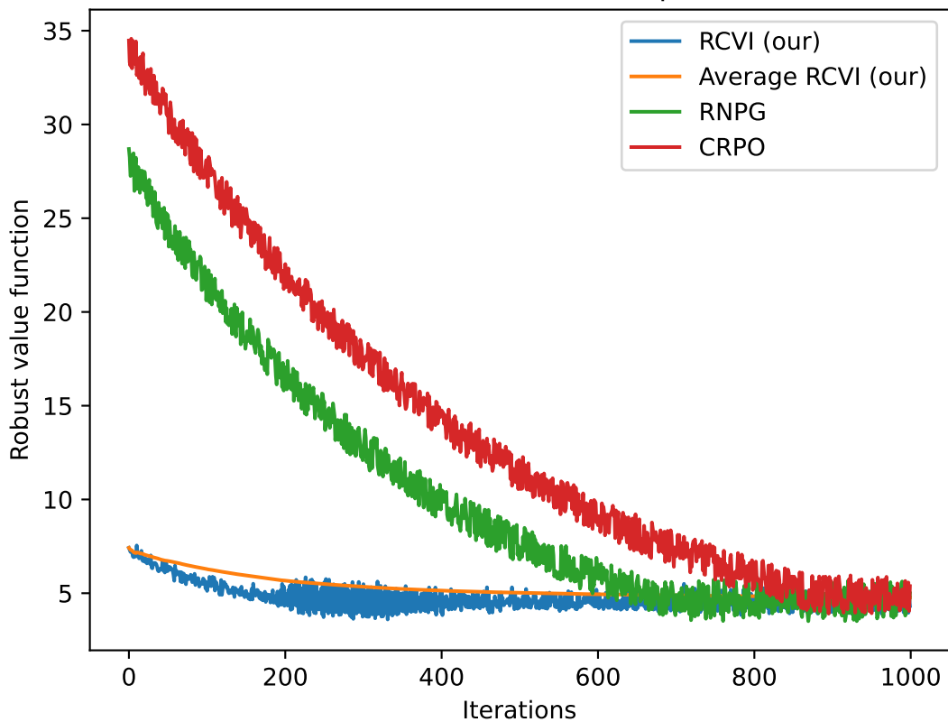
Robust Value function comparison
