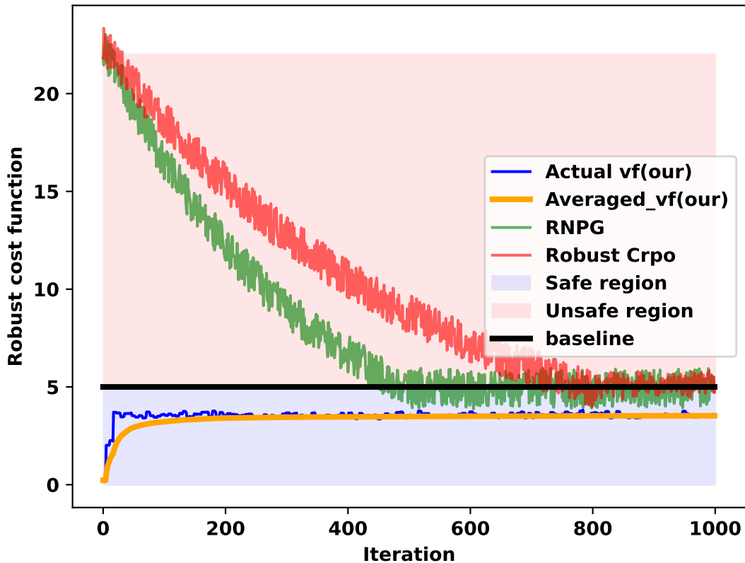
Cost function for RVI in augmented space
