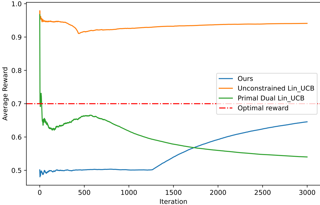
Avg Reward vs Iteration (10 arm) Lookup true reward and true utility
