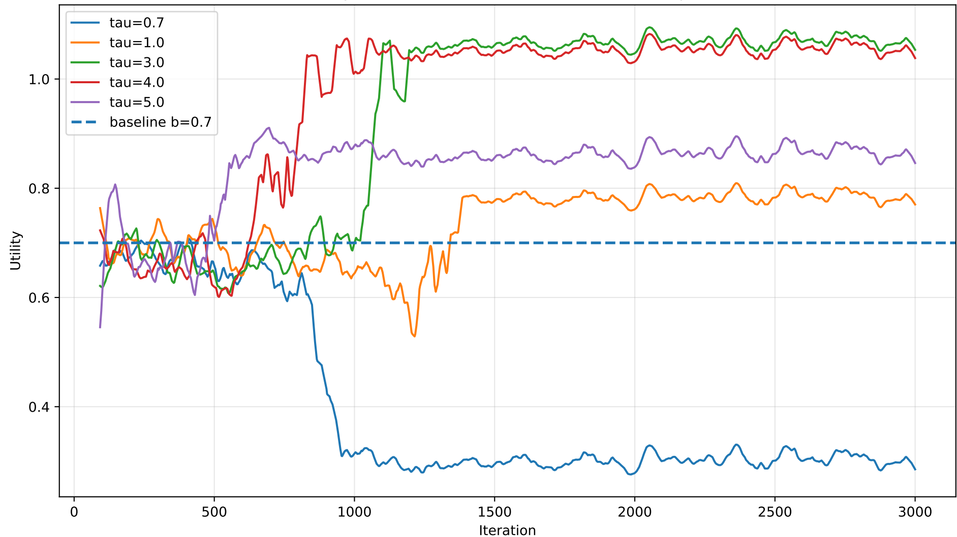
Utility vs Iteration (rho=1.0) — All tau on one plot
