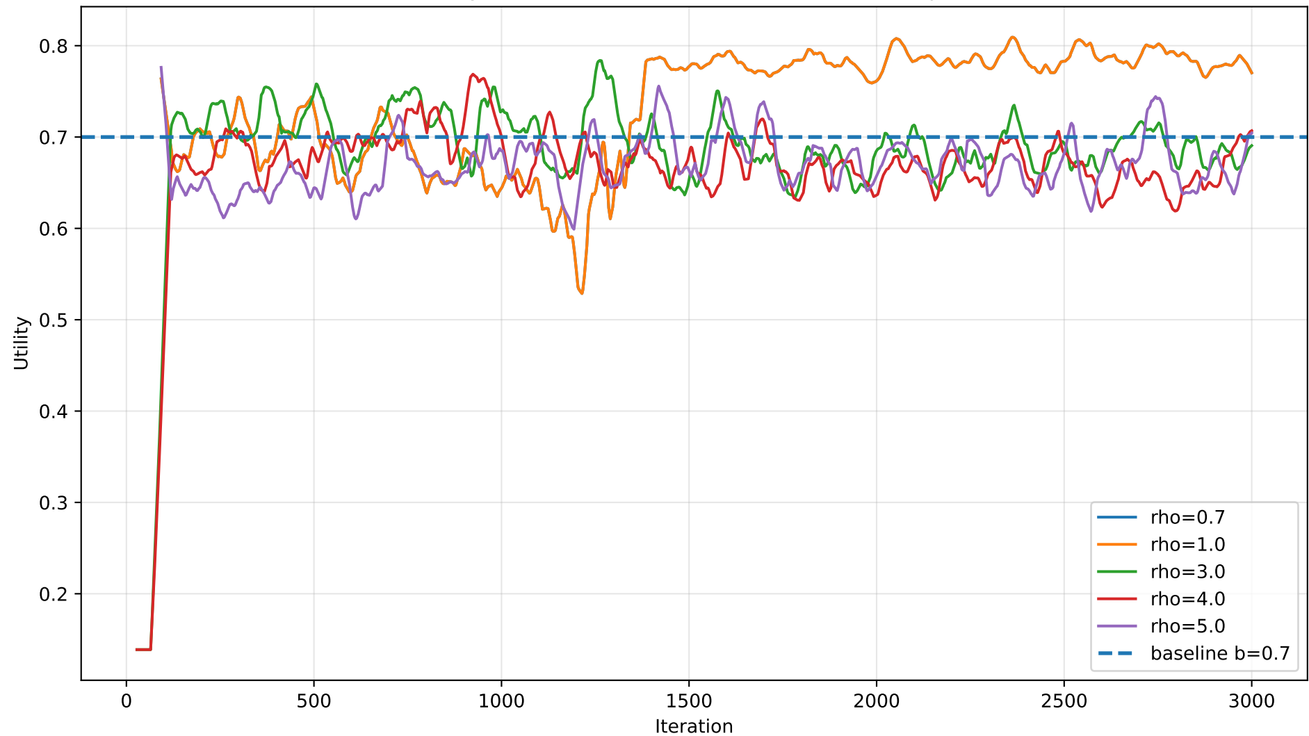
Utility vs Iteration (tau=1.0) — All rho on one plot
