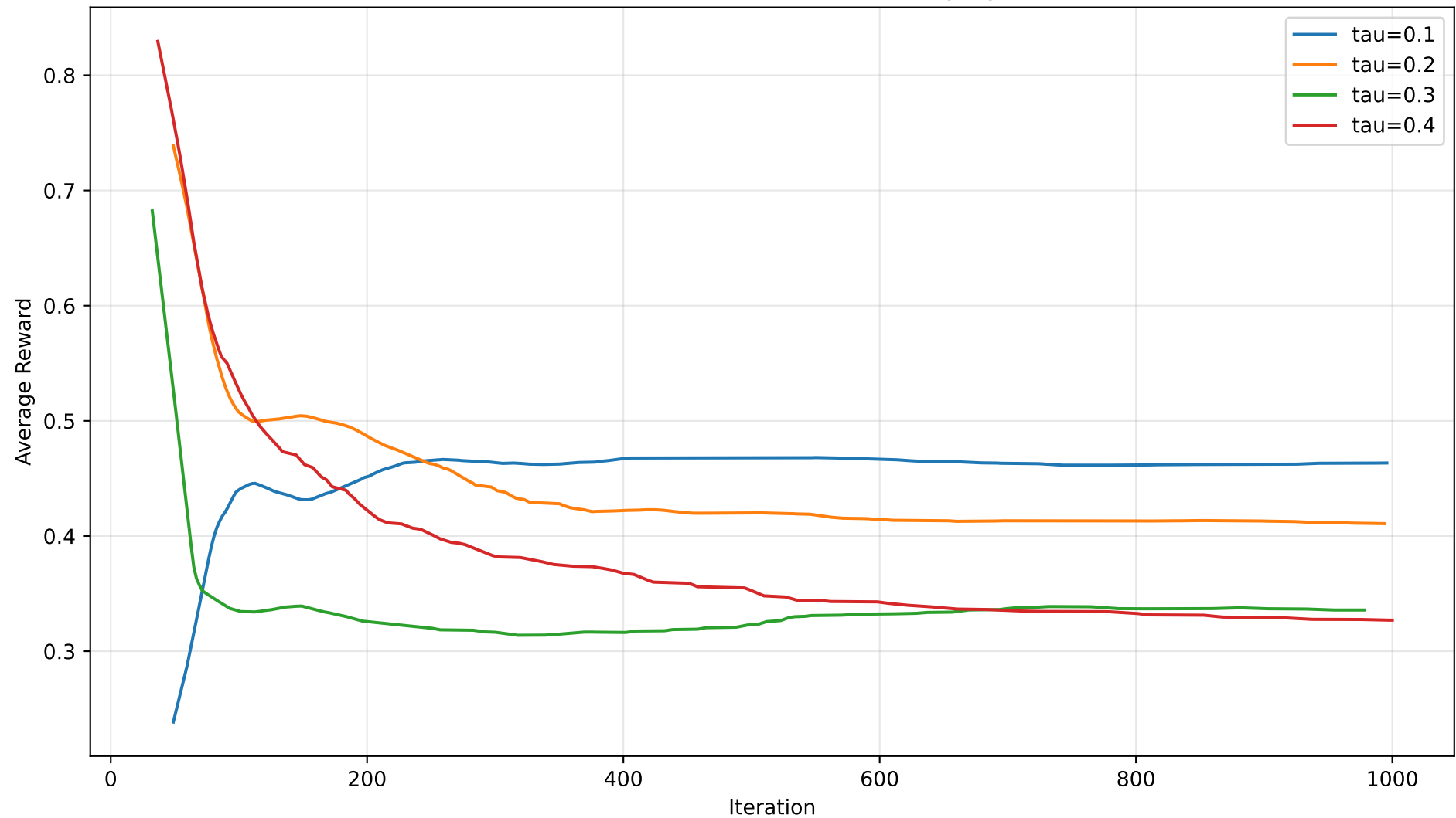
Reward vs Iteration ( \rho=0.3 ) — varying \tau
