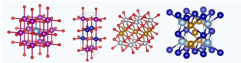
Crystal Structures
