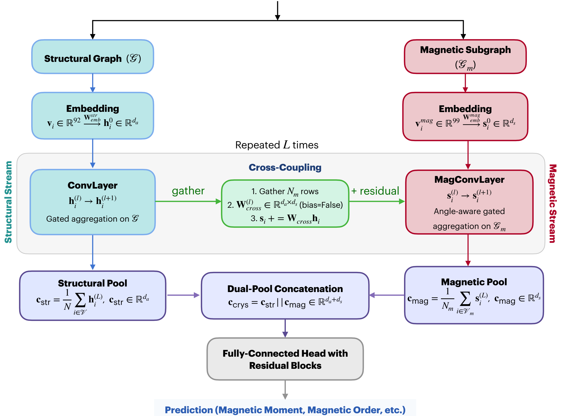
Crystal Structures
