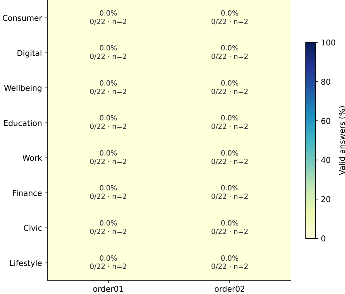
meta-llama-3.1-8b-instruct
