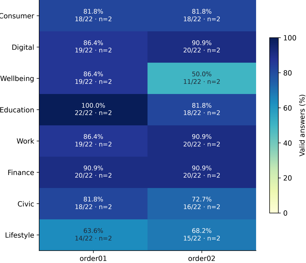
qwen2.5-7b-instruct-1m
