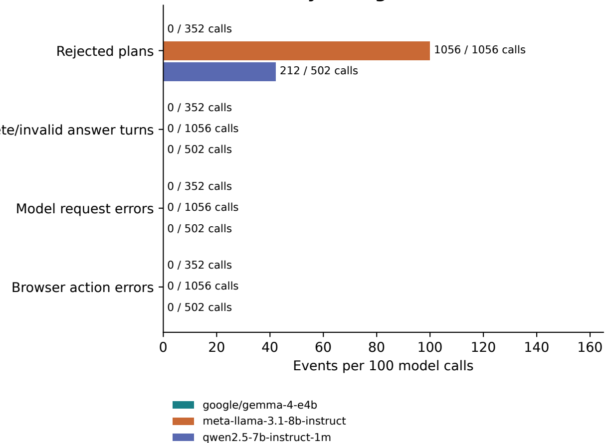
Why the agent retries
