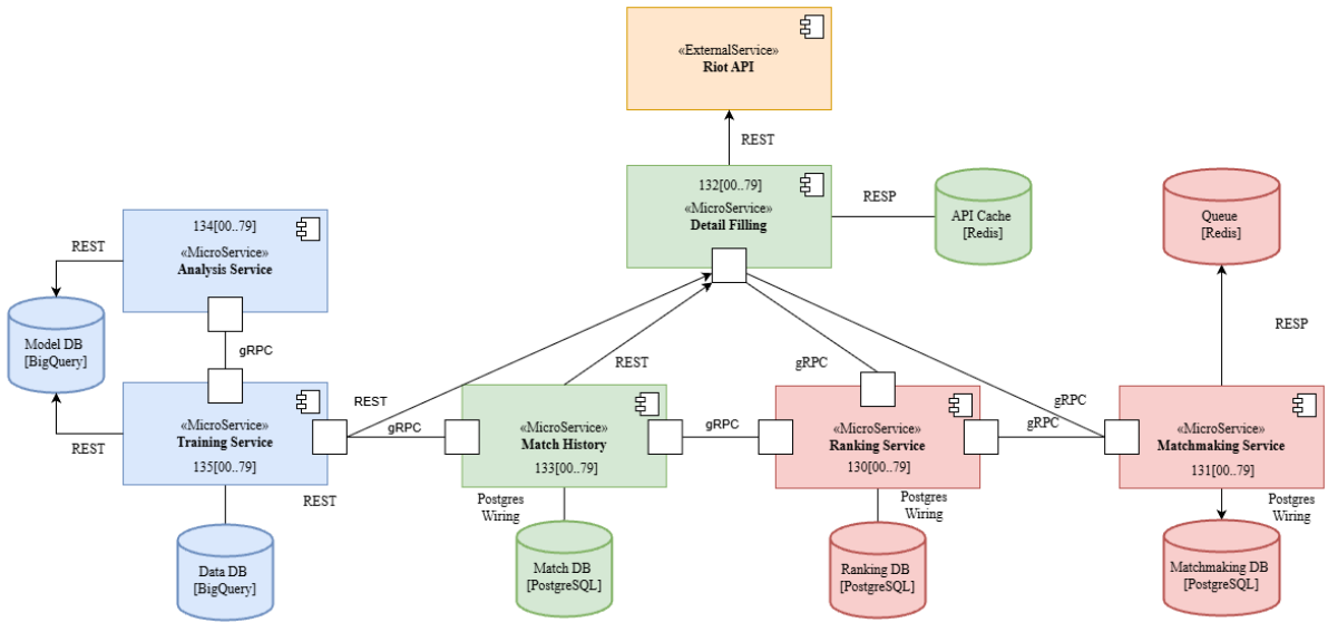
Figure 1: Application Architecture
