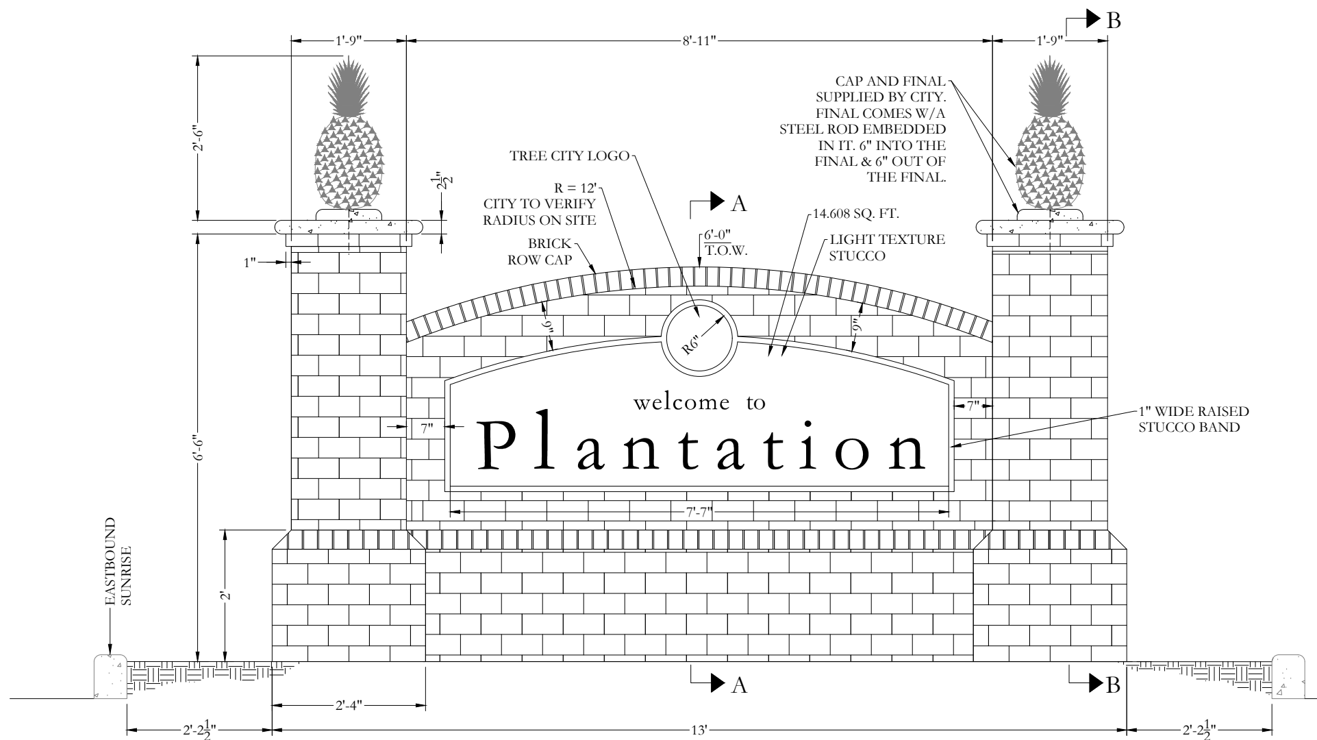
PROPOSED ENTRY SIGN ELEVATION
