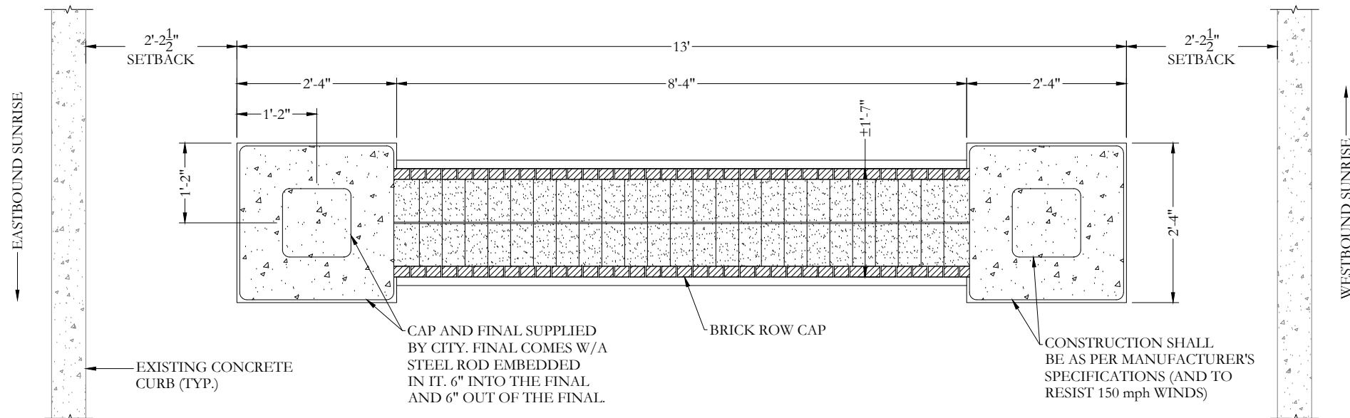
PROPOSED ENTRY SIGN TOP VIEW
