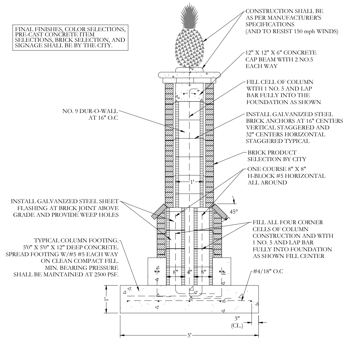
SECTION B-B
