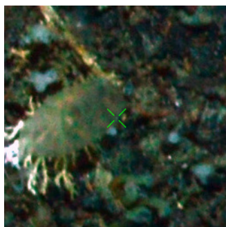
TAN1802_097
