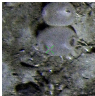
NBP1402_Transect47
