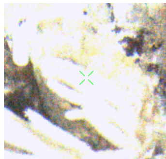
JR17003_027
