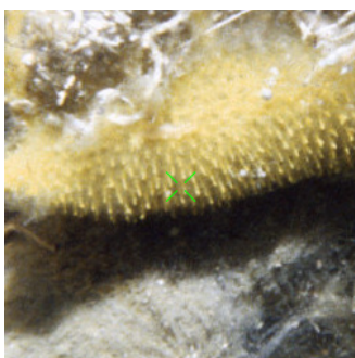
PS14_276
