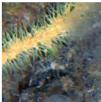
AA2011_CTD97
