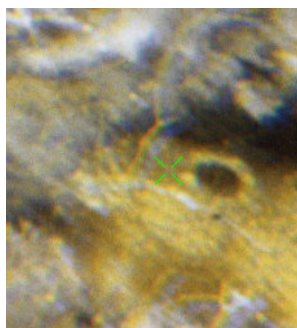
PS14_276
