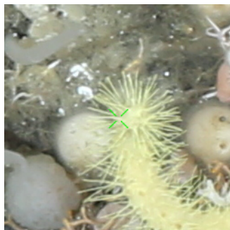
PS96_057
