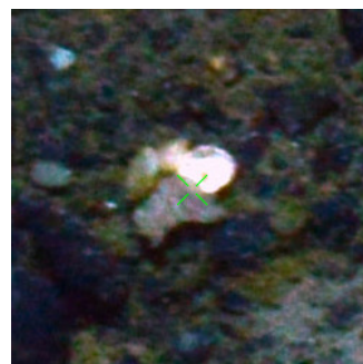
tan1901_168
