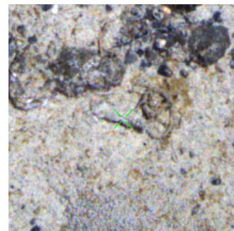
JR17001_MT4
