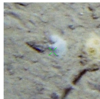
NBP1502_KC5
