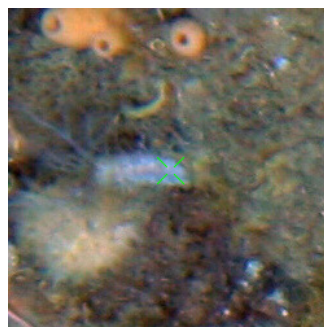
AA2011_CTD97
