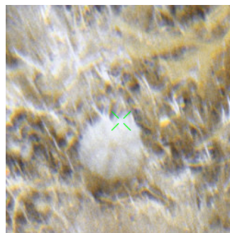
PS18_171
