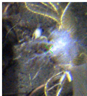
JR17003_028
