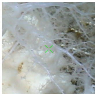
PS96_010
