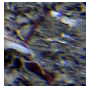
NBP1502_KC3
