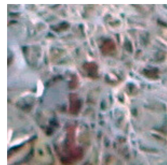
AA2011_CTD68
