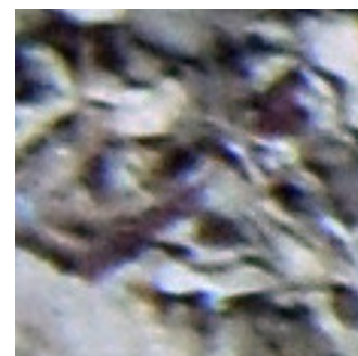
NBP1502_KC3
