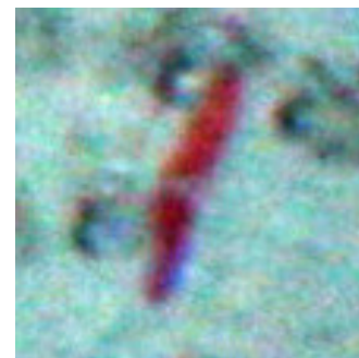
PS81_204
