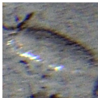
NBP1502_KC6
