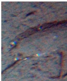
CRS_1276
