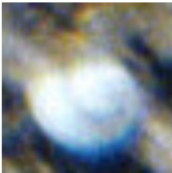
PS18_175
