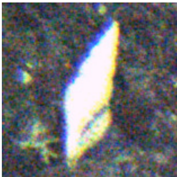
JR15005_117
