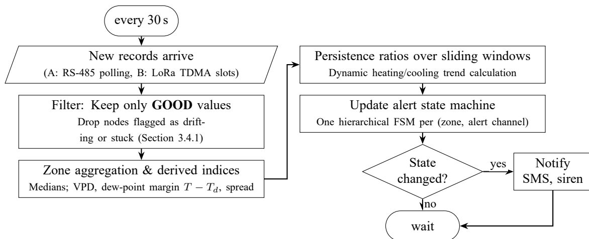
Figure 4.1: Alert analysis pipeline on the gateway
