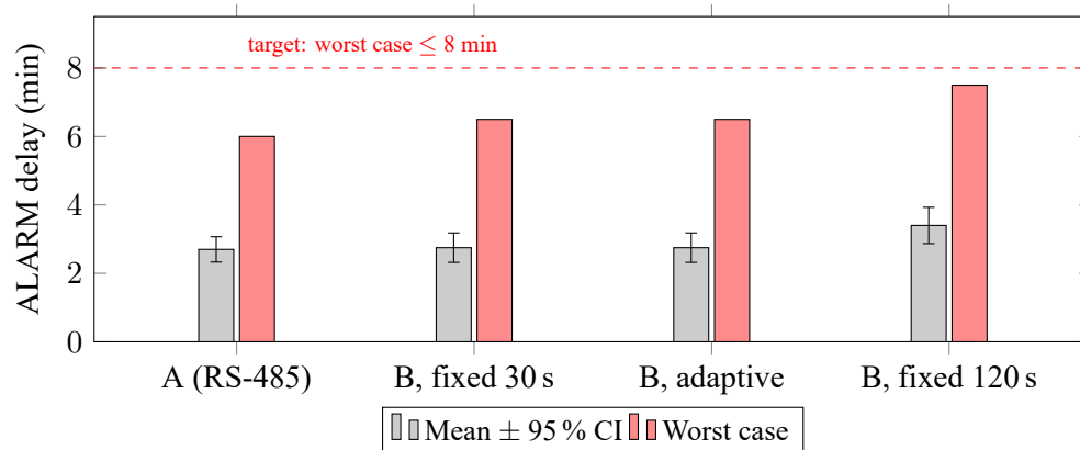
Figure 5.1: Alert delay with the trend alert switched off (isolates the effect of the network)
