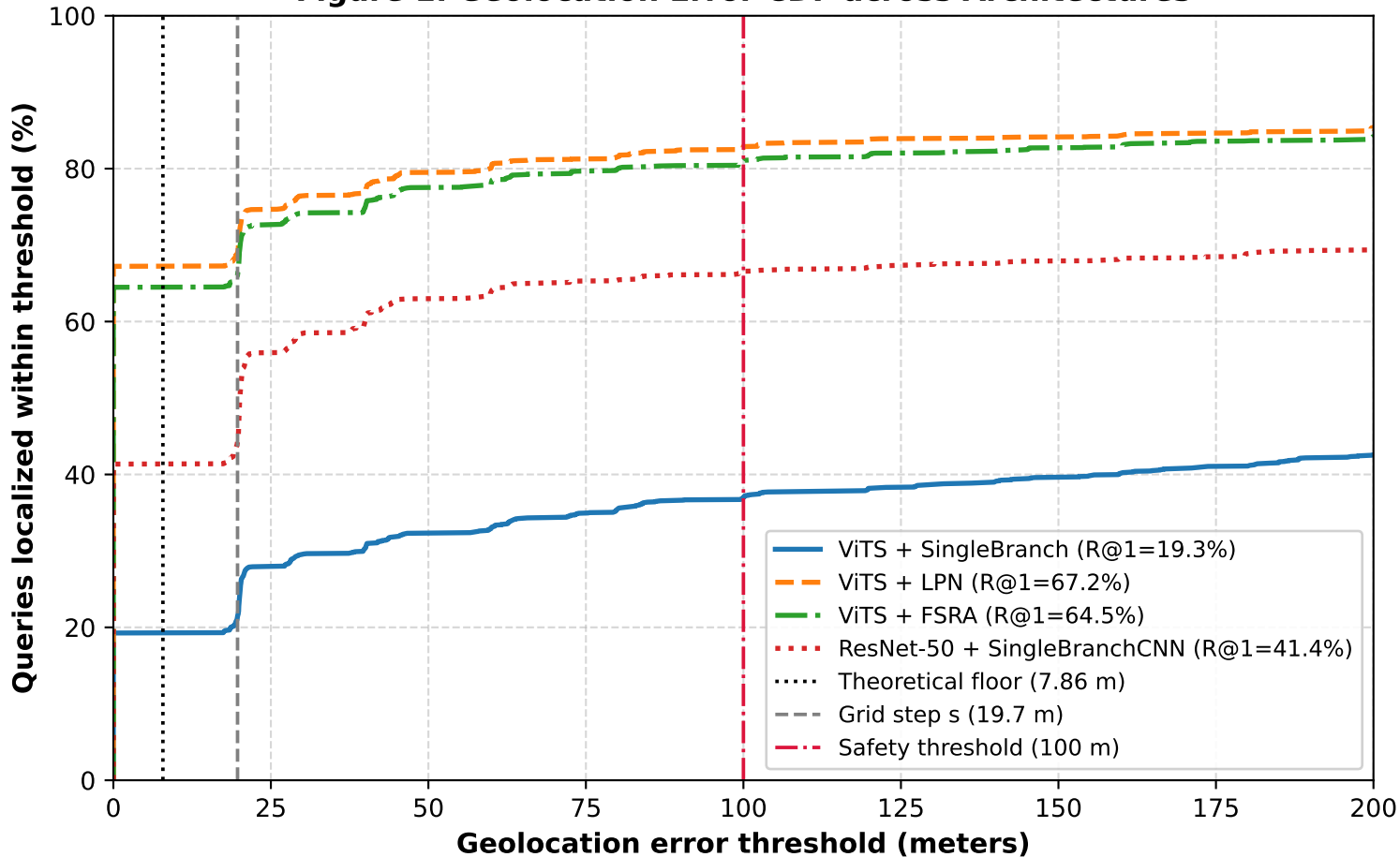
Figure 1: Geolocation Error CDF across Architectures
