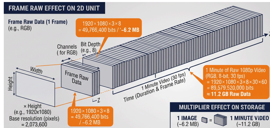
Figure 04: Raw image and video size grow from the combined effects of resolution, channel count, bit depth, frame rate, and duration. Video becomes large because it extends image data through time.
