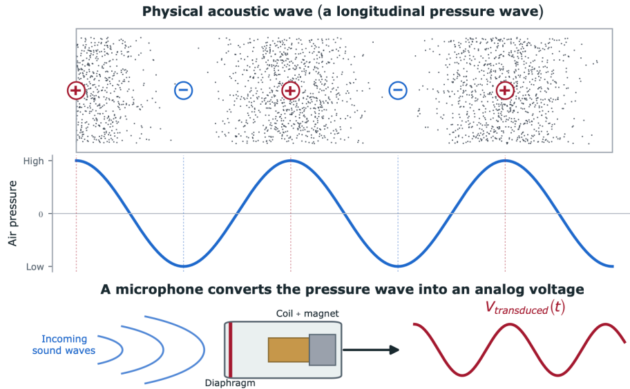
Figure 01: The Mechanical and Electrical Transduction of a Sound Wave. Physically, sound is a longitudinal pressure wave, transduced into a continuous analog electrical signal.
