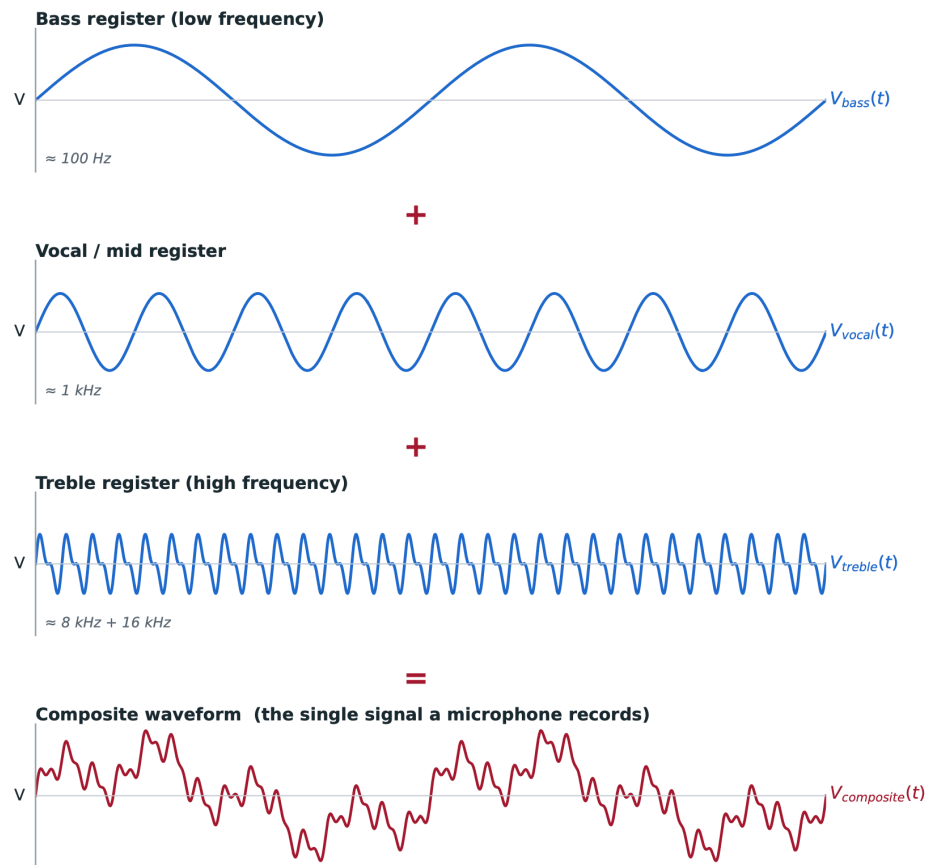
Figure 02: The Superposition Principle and Composite Wave Mechanics - Algebraic Summation of Independent Frequencies into a Single Waveform
