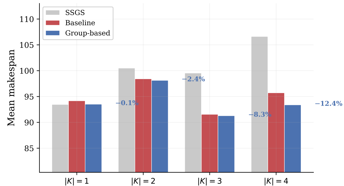
(b) Mean makespan (feasible instances)
