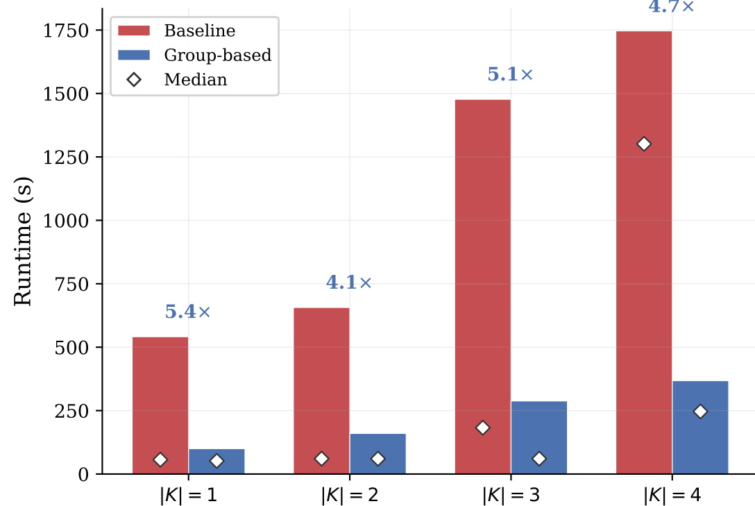
(c) Mean and median runtime
