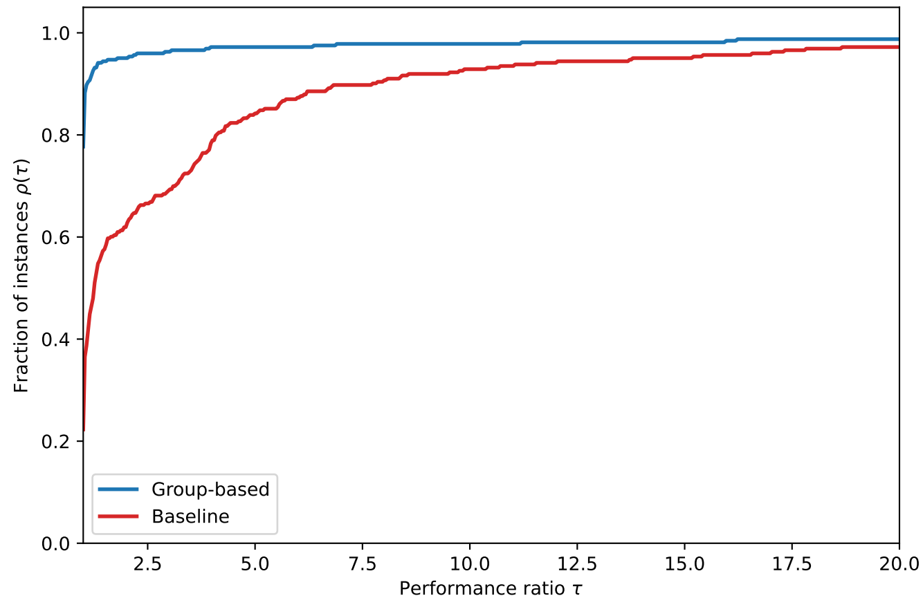
(A) Performance Profile
