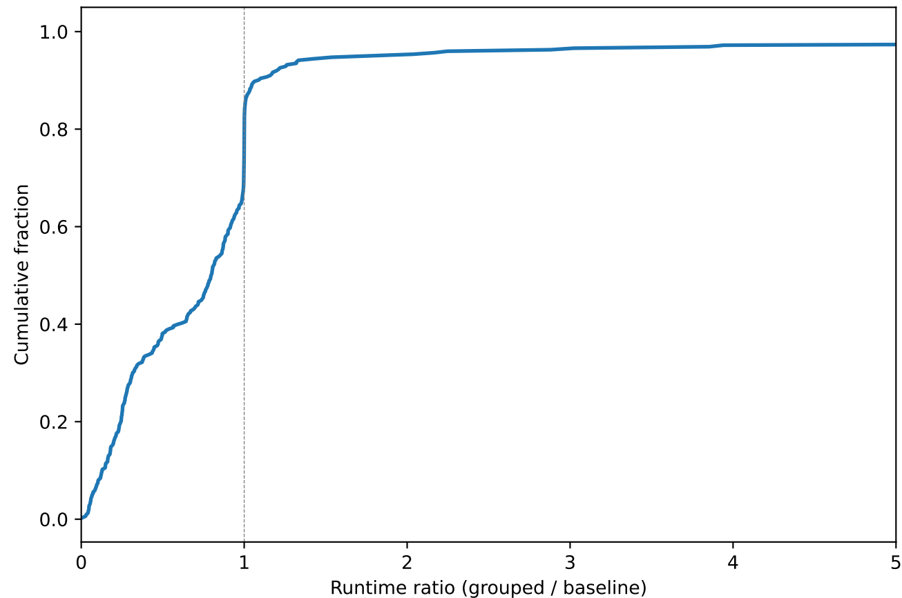
(B) CDF of Runtime Ratio
