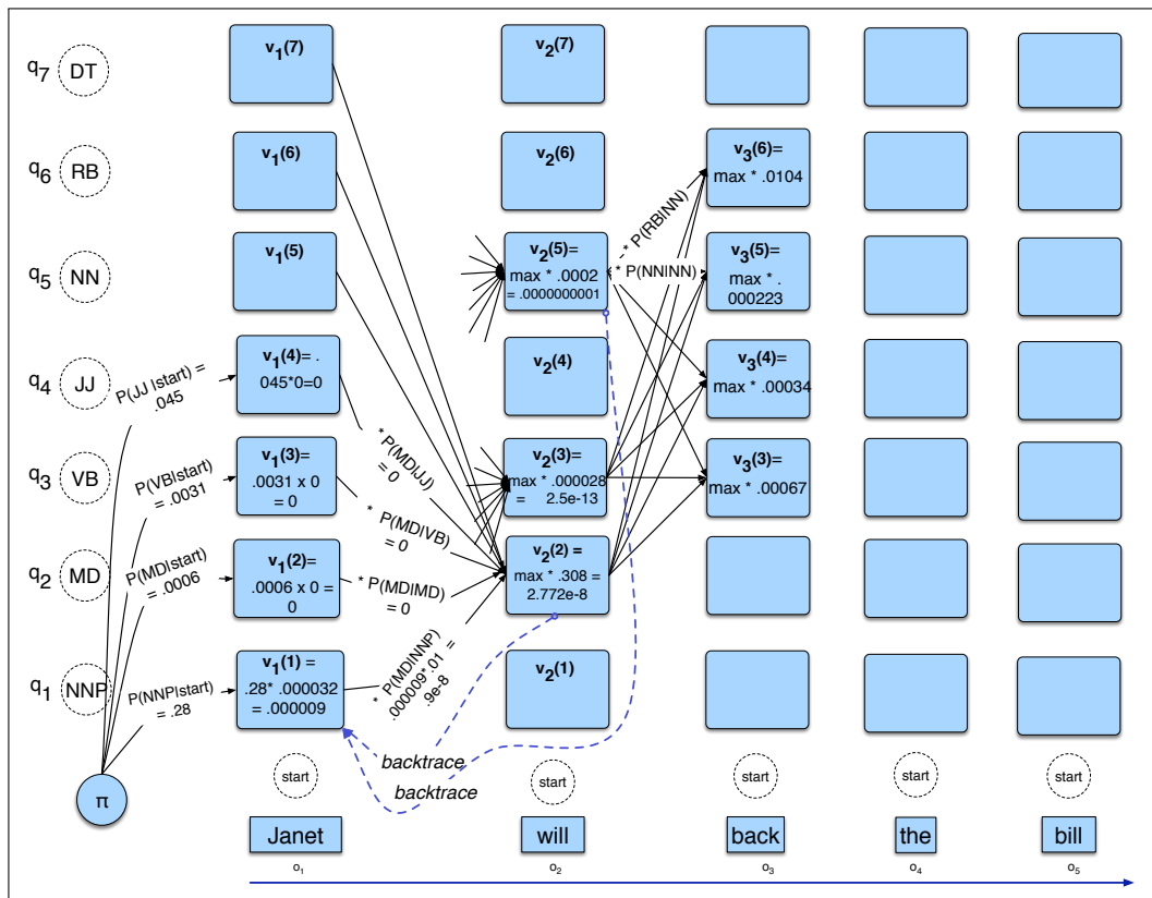
Figure 18.14 The first few entries in the individual state columns for the Viterbi algorithm. Each cell keeps the probability of the best path so far and a pointer to the previous cell along that path. We have only filled out columns 1 and 2; to avoid clutter most cells with value 0 are left empty. The rest is left as an exercise for the reader. After the cells are filled in, backtracing from the end state, we should be able to reconstruct the correct state sequence NNP MD VB DT NN.
