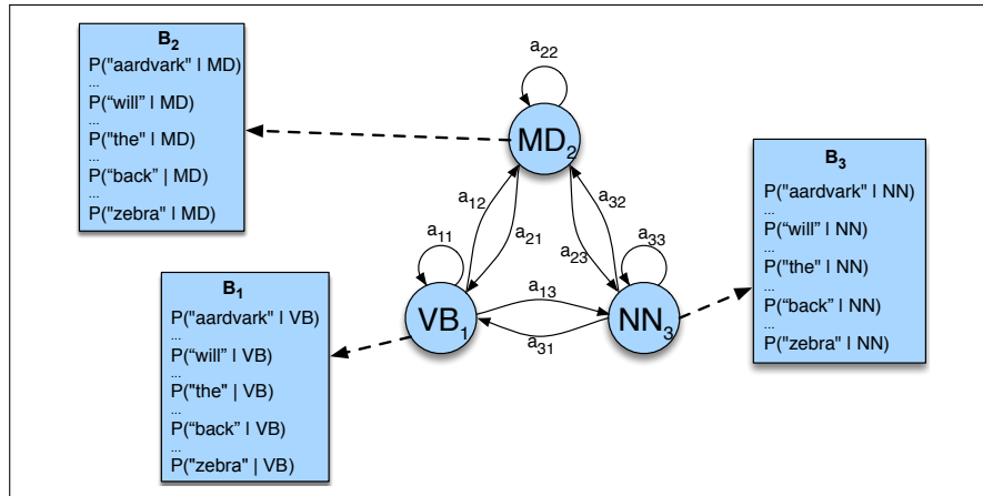
Figure 18.9 An illustration of the two parts of an HMM representation: the A transition probabilities used to compute the prior probability, and the B observation likelihoods that are associated with each state, one likelihood for each possible observation word.
