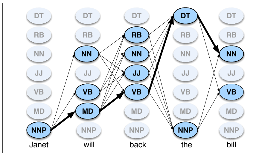
Figure 18.11 A sketch of the lattice for Janet will back the bill , showing the possible tags ( q_i ) for each word and highlighting the path corresponding to the correct tag sequence through the hidden states. States (parts of speech) which have a zero probability of generating a particular word according to the B matrix (such as the probability that a determiner DT will be realized as Janet ) are greyed out.
