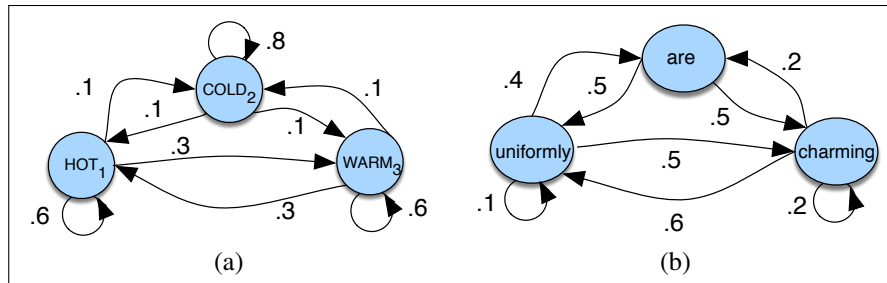
Figure 18.8 A Markov chain for weather (a) and one for words (b), showing states and transitions. A start distribution \pi is required; setting \pi = [0.1, 0.7, 0.2] for (a) would mean a probability 0.7 of starting in state 2 (cold), probability 0.1 of starting in state 1 (hot), etc.
