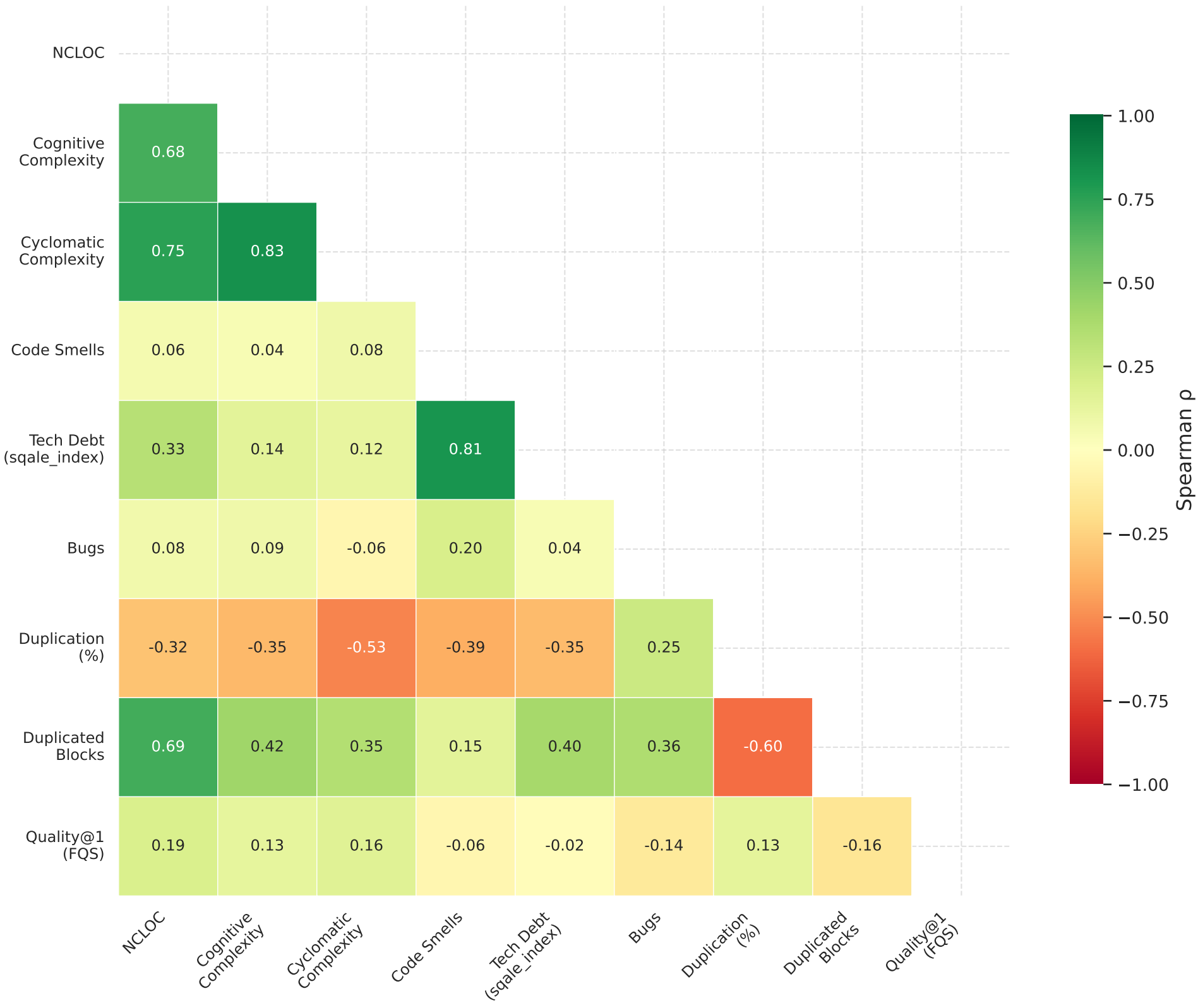
Spearman Correlation Matrix of Software Quality Metrics (all models and strategies combined)
