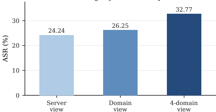
Leakage by observer scope
