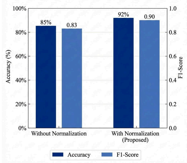
Fig. 6: Effect of Semantic Normalization
