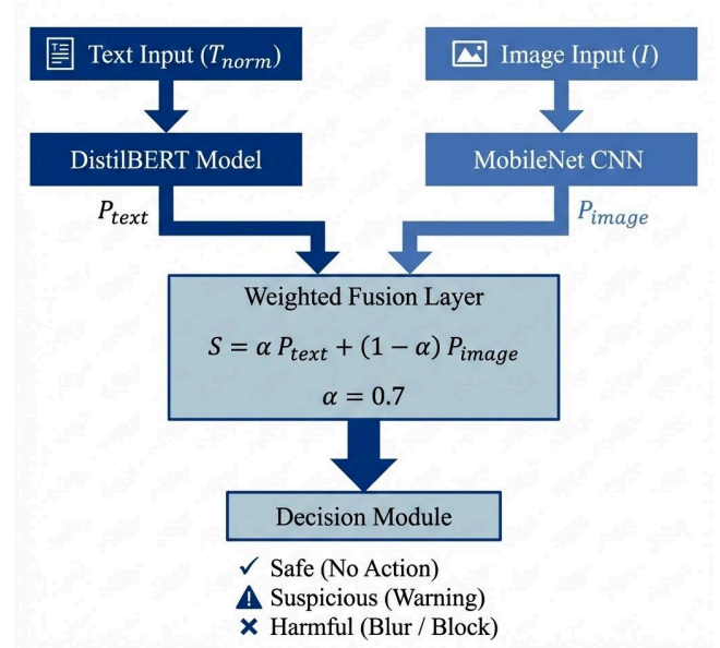
Fig. 3 : Multimodal Fusion Strategy
