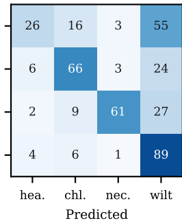
(b) Shifted
