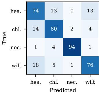
(a) In-domain
