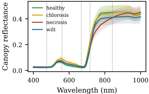
(a) VNIR; RedEdge-MX centers dotted
