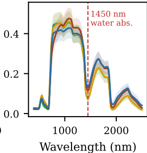
(b) Full 400–2500 nm
