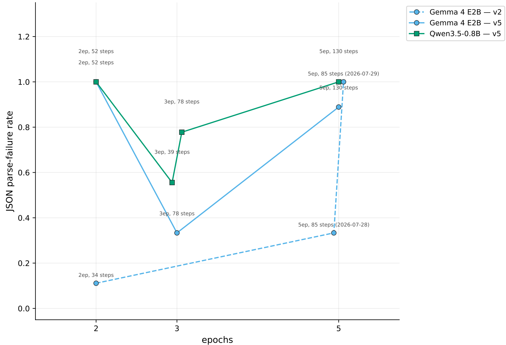
JSON parse-failure rate vs. epoch count
