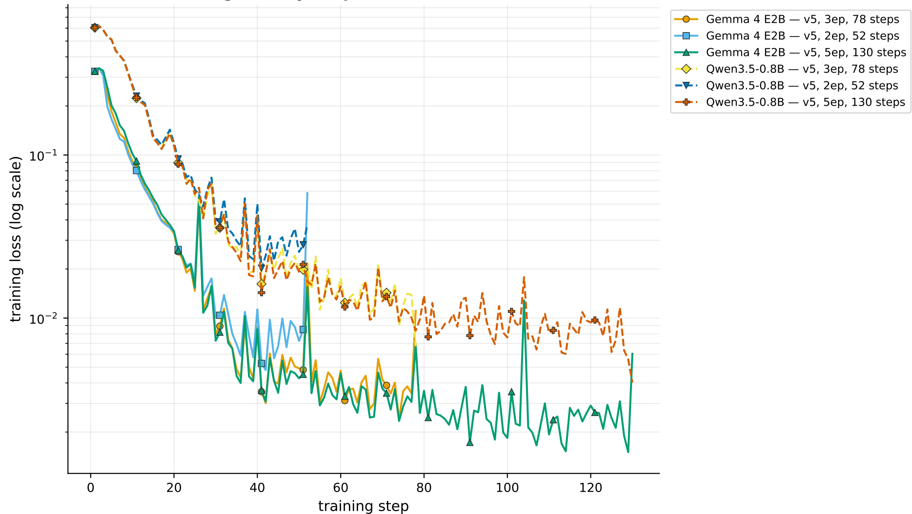
Training loss by step, across fine-tune runs
