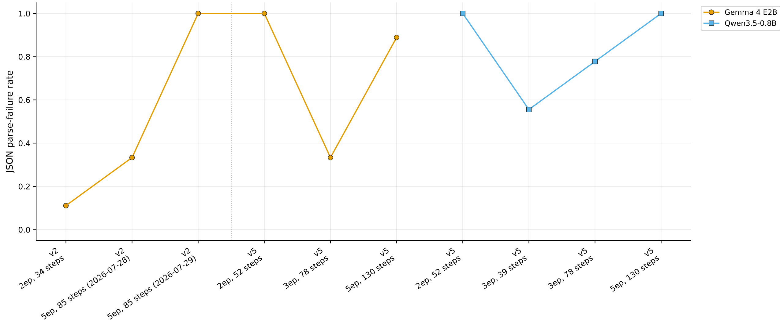
JSON parse-failure rate across fine-tune runs
