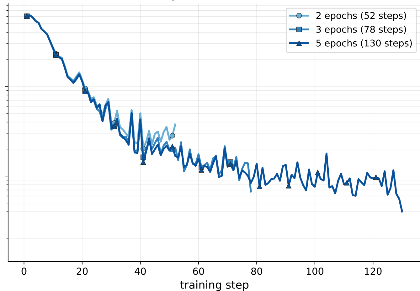
Qwen3.5-0.8B
