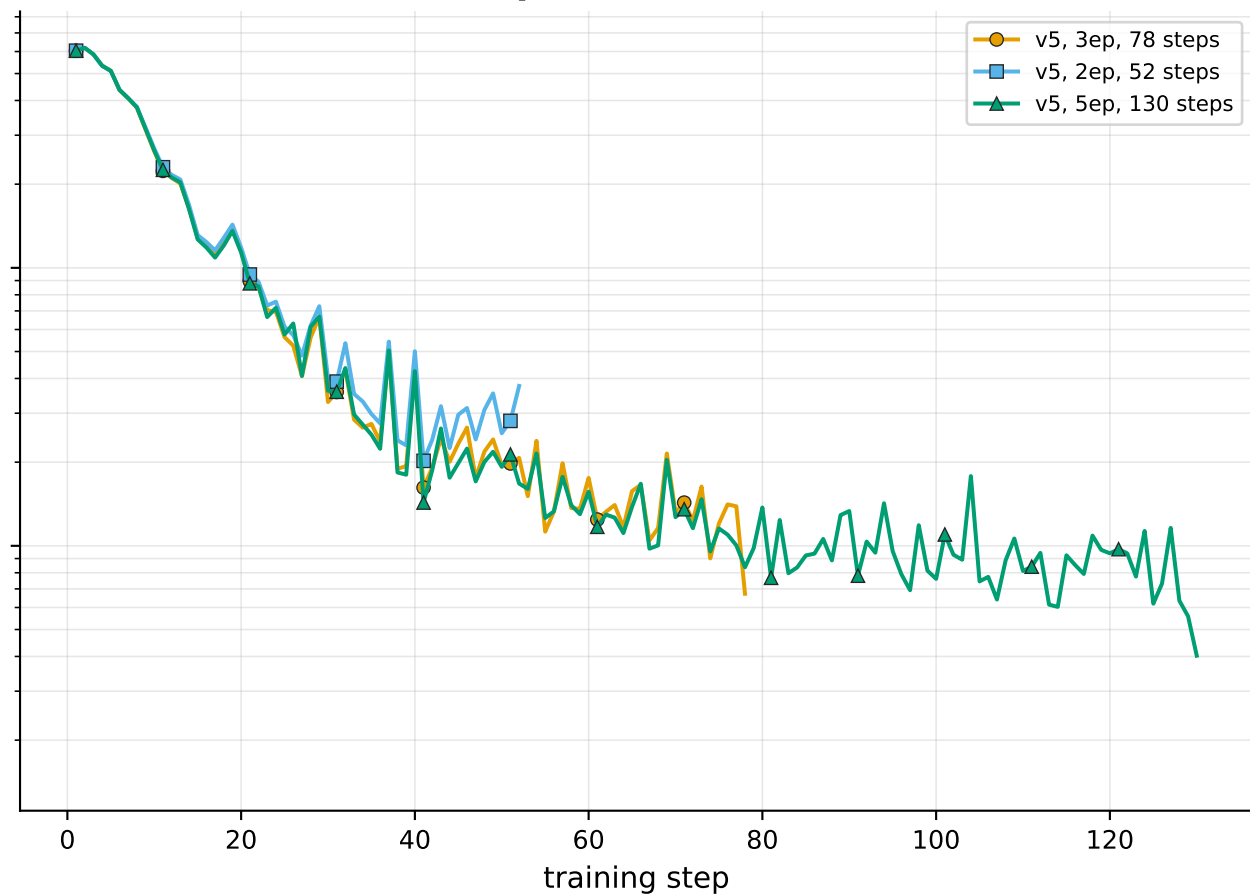
Qwen3.5-0.8B
