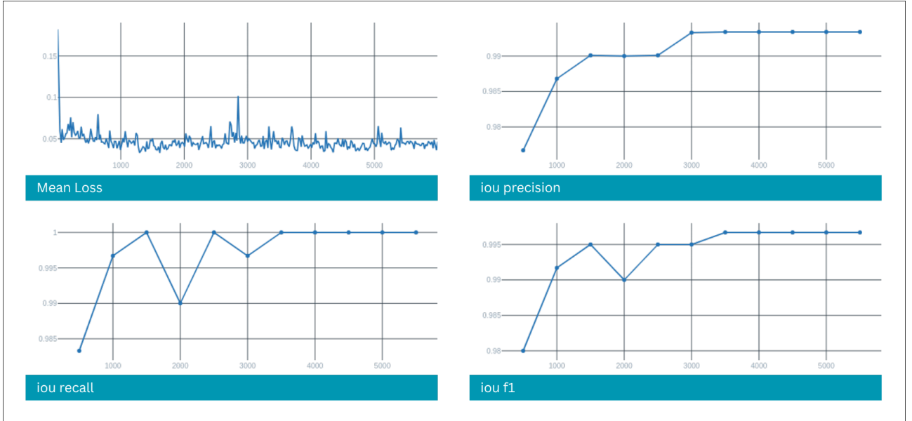
Figure 4.5: Illustration of the recall, precision, and the intersection over union (IOU) performance of the CRAFT model with 5000 steps.
