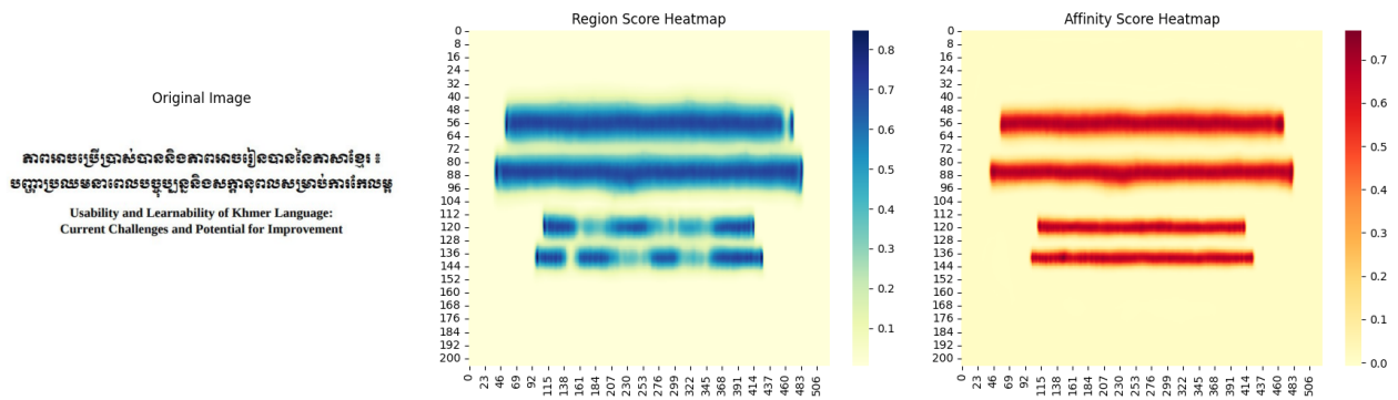
Figure 5.2: Headmap visualization of Region score and Affinity score of CRAFT model on Khmer text.
