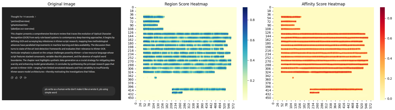
Figure 5.1: Headmap visualization of Region score and Affinity score of CRAFT model on English text.
