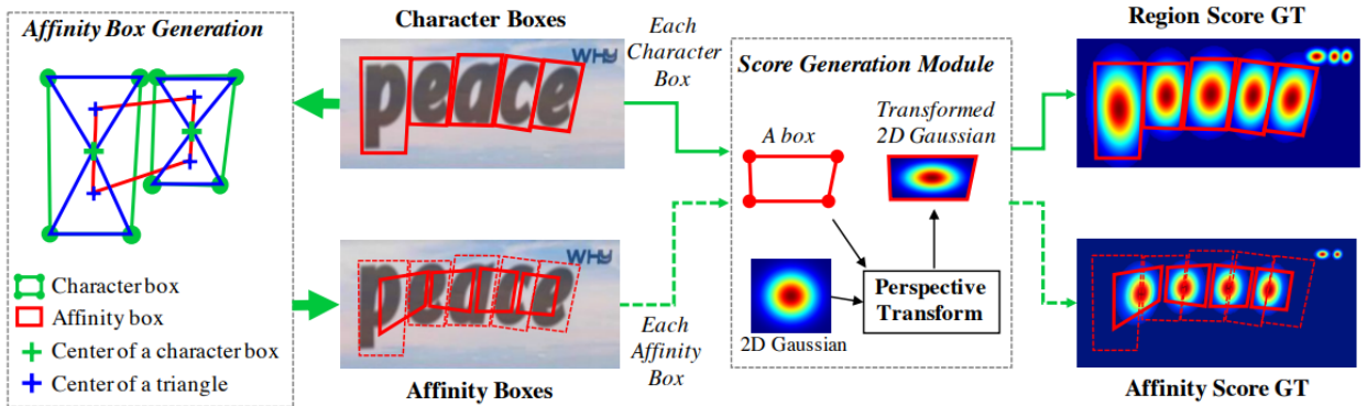
Figure 4.2: Illustration of ground truth generation procedure in our framework. We generate ground truth labels from a synthetic image that has character level annotations. ( Baek et al., 2019b )
