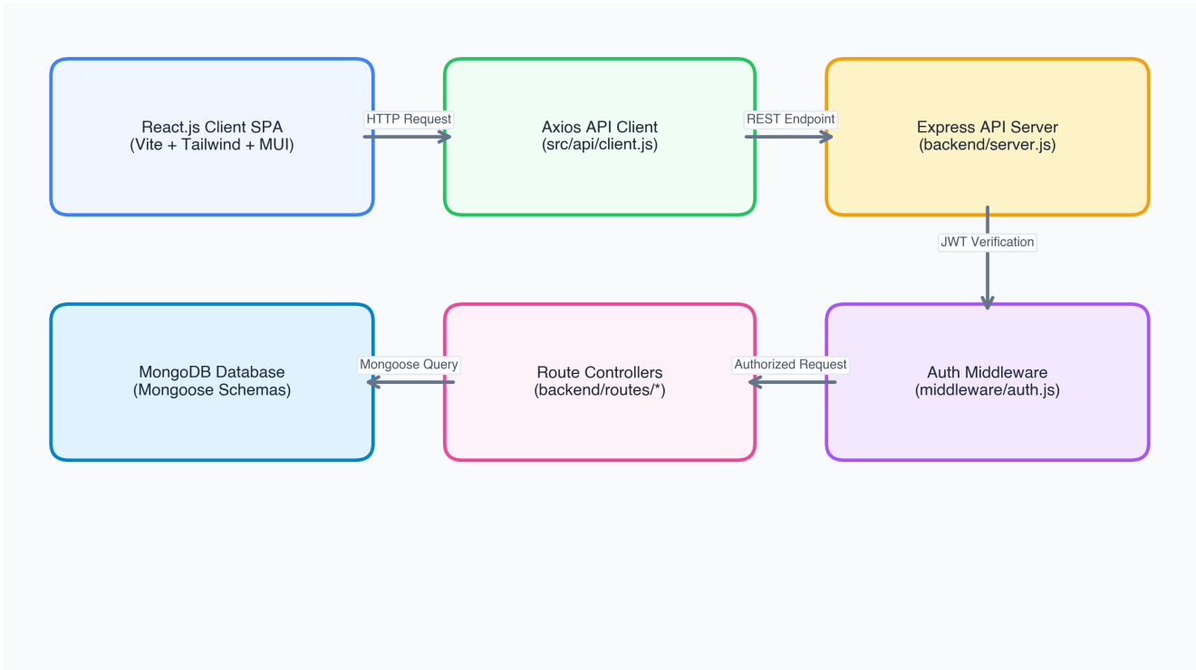
SpacECE Smart Parenting Portal — System Architecture & Data Flow
