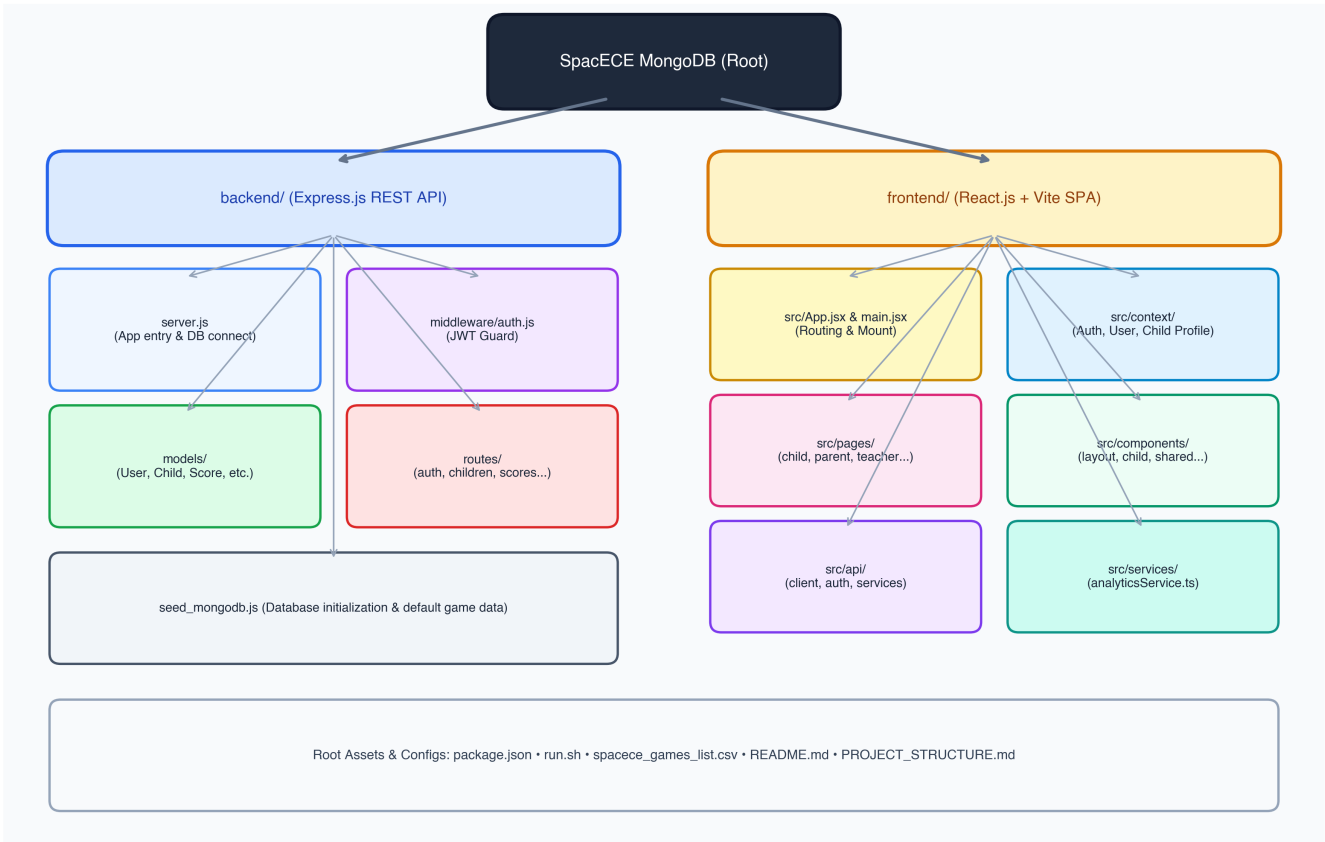
SpacECE MongoDB — Complete Visual File Skeleton & Module Tree
