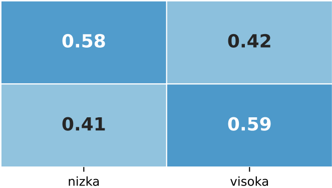
HeteroGCN-MLP-w
