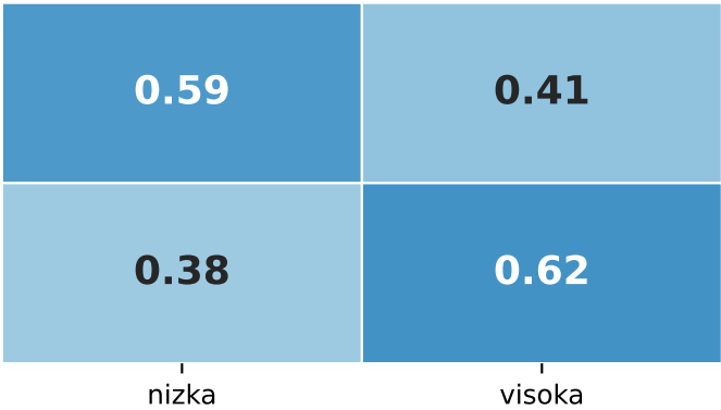
HeteroGCN-mean
