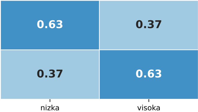
GazeMAE/MOMENT
