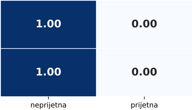
LightGBM
