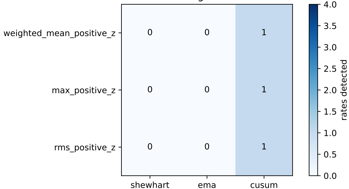
Maximum attack-rate coverage with zero clean alerted nodes
