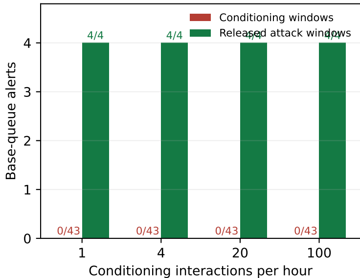
Base detector: conditioning missed, payload retained
