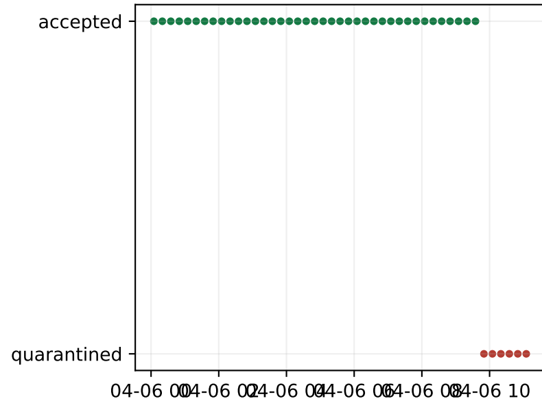
Memory-update decisions
