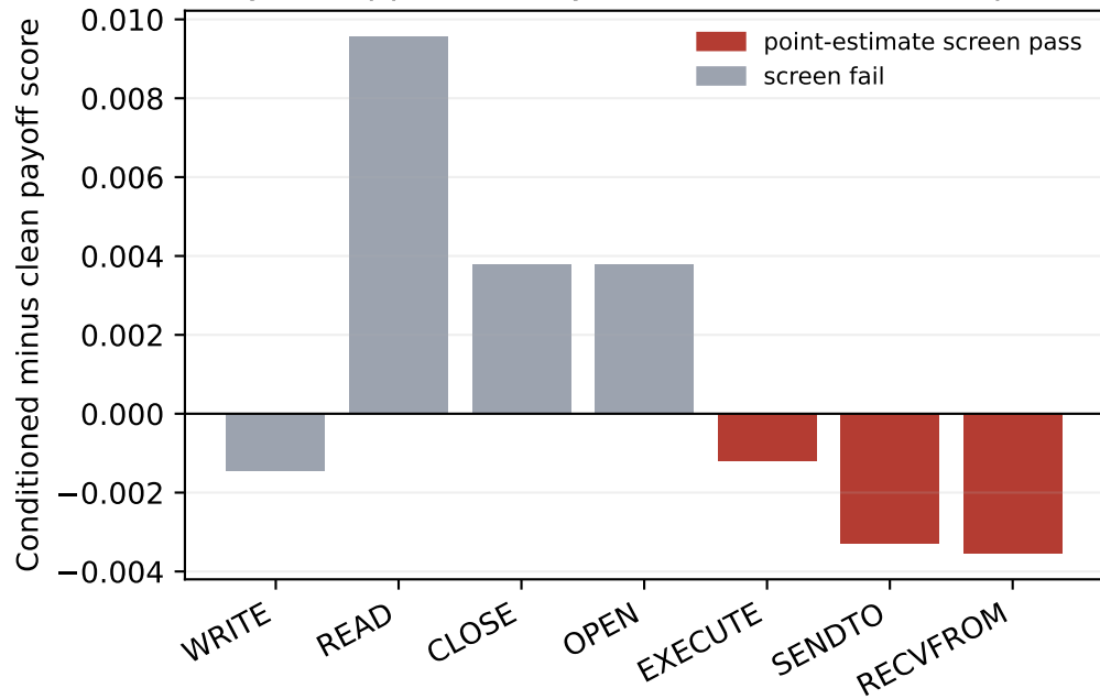
Payoff suppression by observed relation template
