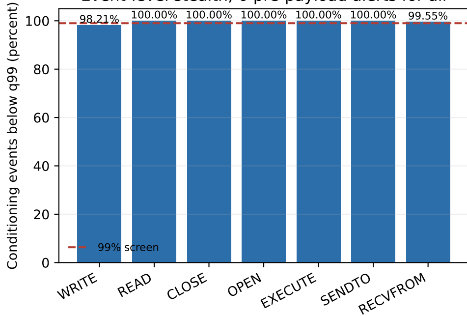
Event-level stealth; 0 pre-payload alerts for all
