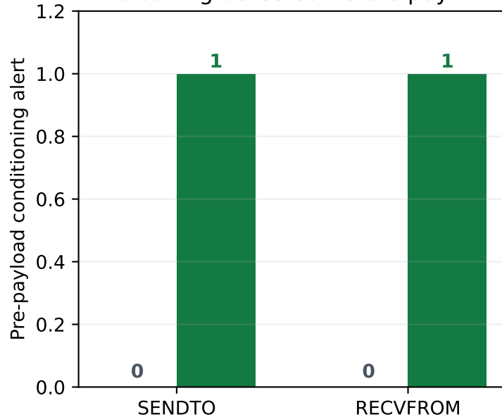
Poisoning detected before payoff
