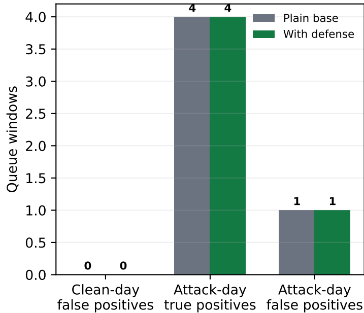
Ordinary operating point preserved
